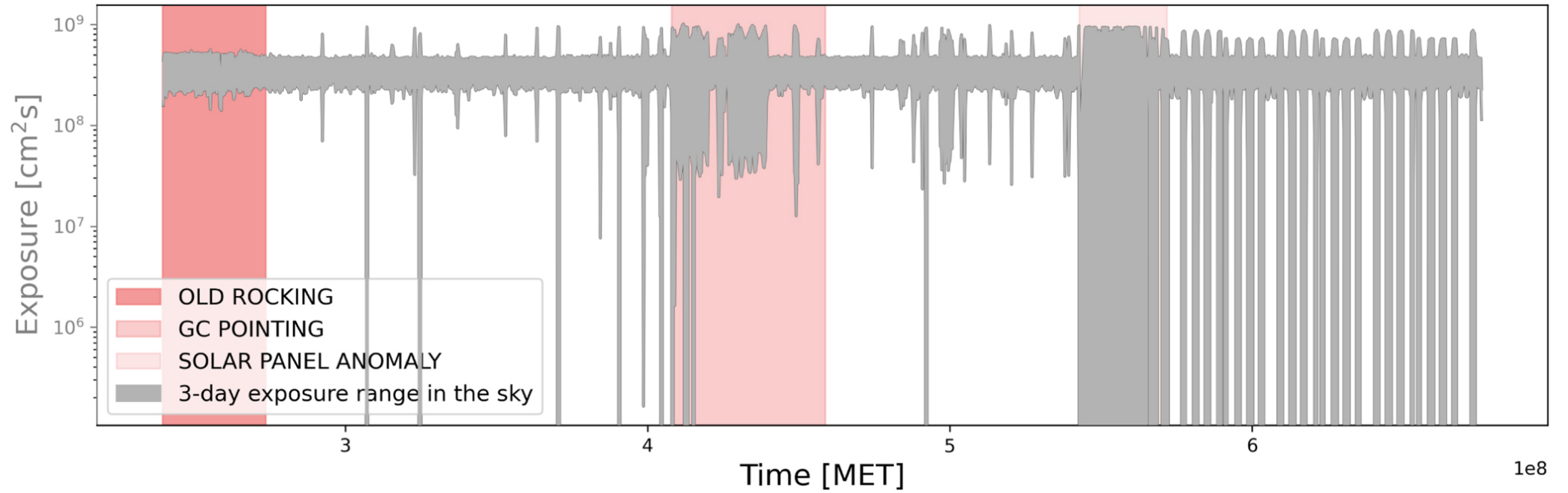
Figure 5. from S. Abdollahi et al 2023 Astrophys. J. Suppl. 265 doi:10.3847/1538-4365/acbb6a https://dx.doi.org/10.3847/1538-4365/acbb6a © 2023. The Author(s). Published by the American Astronomical Society.
