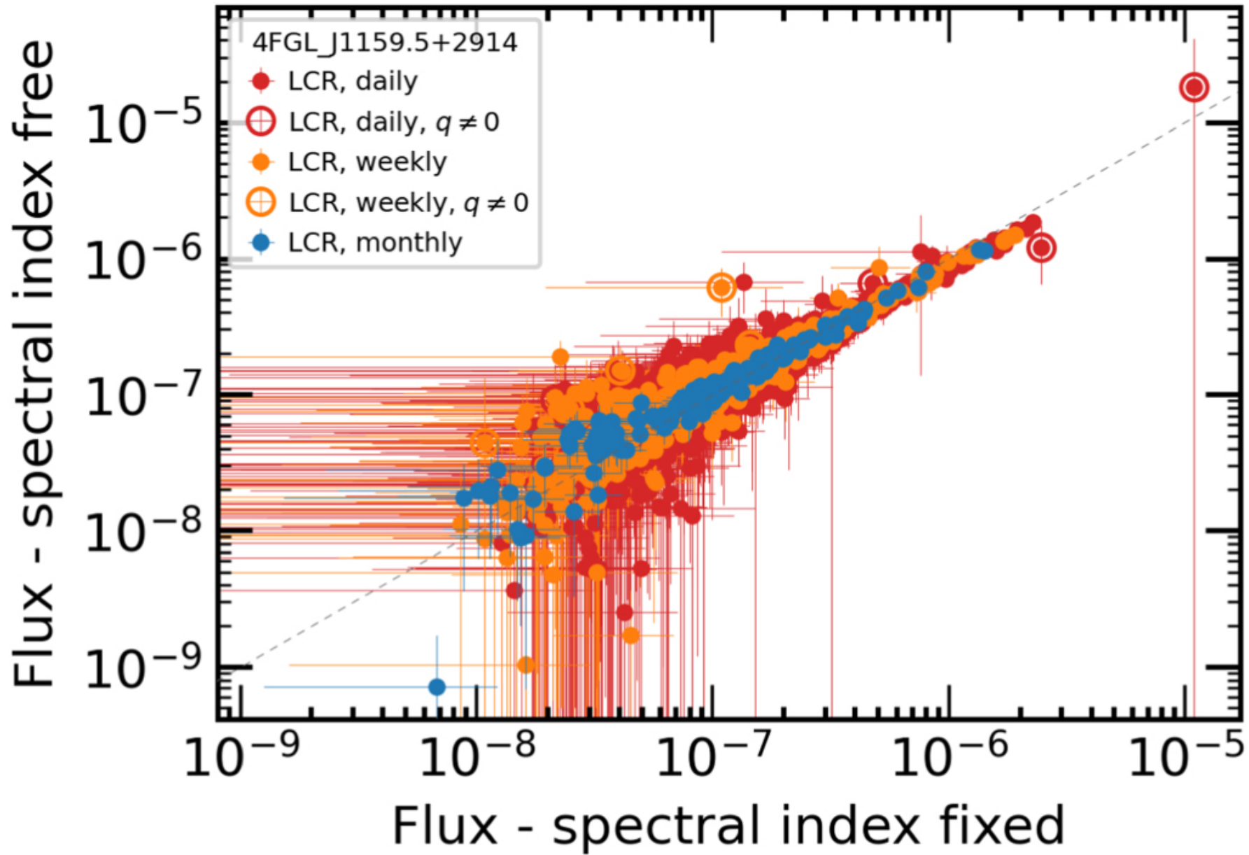
Figure 4. from S. Abdollahi et al 2023 Astrophys. J. Suppl. 265 doi:10.3847/1538-4365/acbb6a https://dx.doi.org/10.3847/1538-4365/acbb6a © 2023. The Author(s). Published by the American Astronomical Society.
