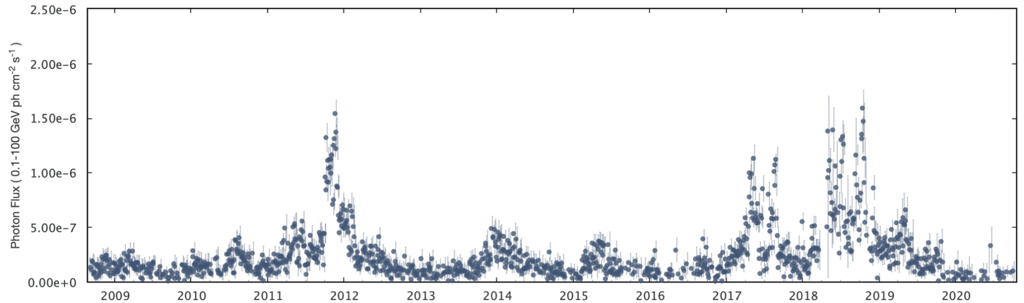
Figure 3. from S. Abdollahi et al 2023 Astrophys. J. Suppl. 265 doi:10.3847/1538-4365/acbb6a https://dx.doi.org/10.3847/1538-4365/acbb6a © 2023. The Author(s). Published by the American Astronomical Society.
