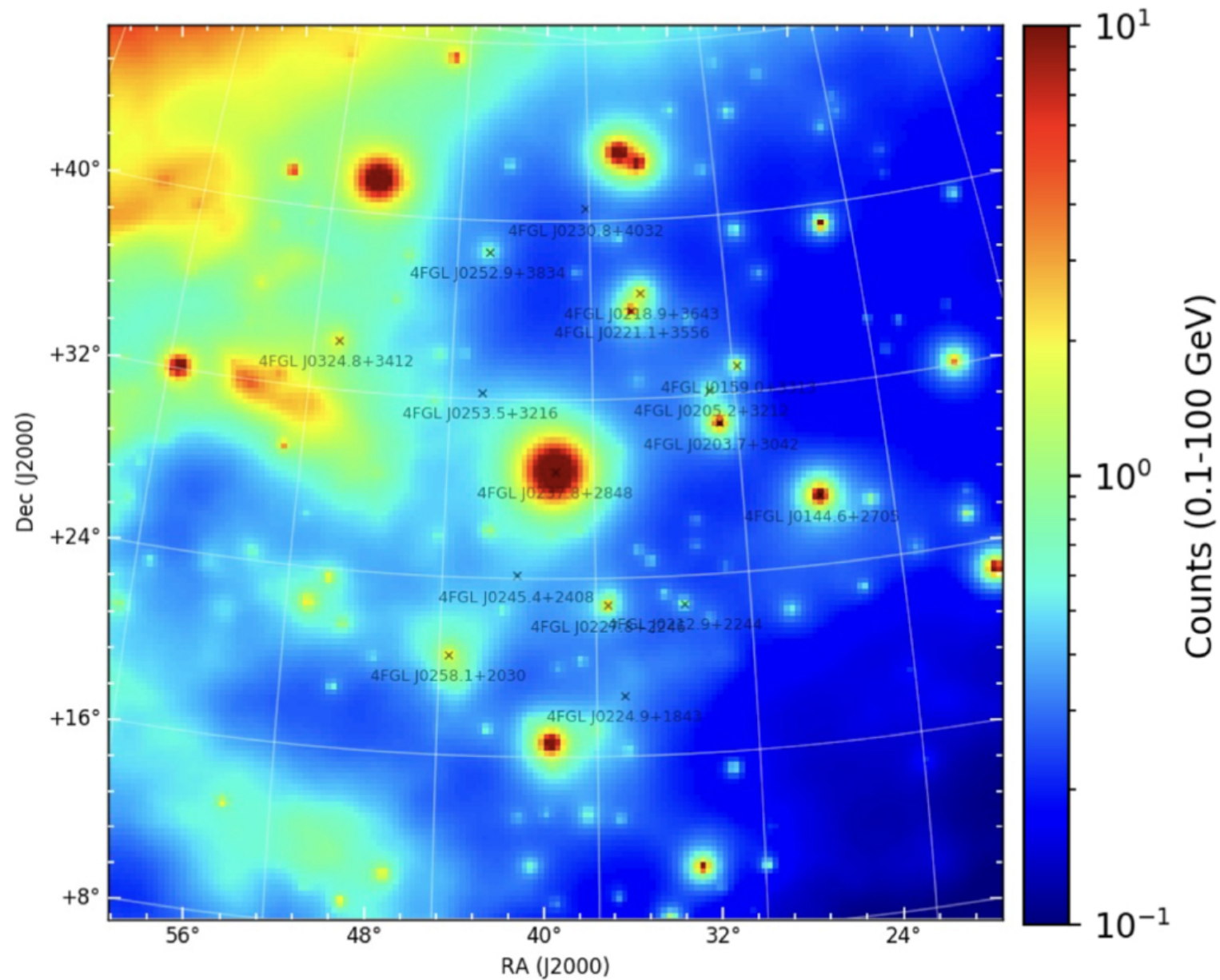
Figure 2. from S. Abdollahi et al 2023 Astrophys. J. Suppl. 265 doi:10.3847/1538-4365/acbb6a https://dx.doi.org/10.3847/1538-4365/acbb6a © 2023. The Author(s). Published by the American Astronomical Society.
