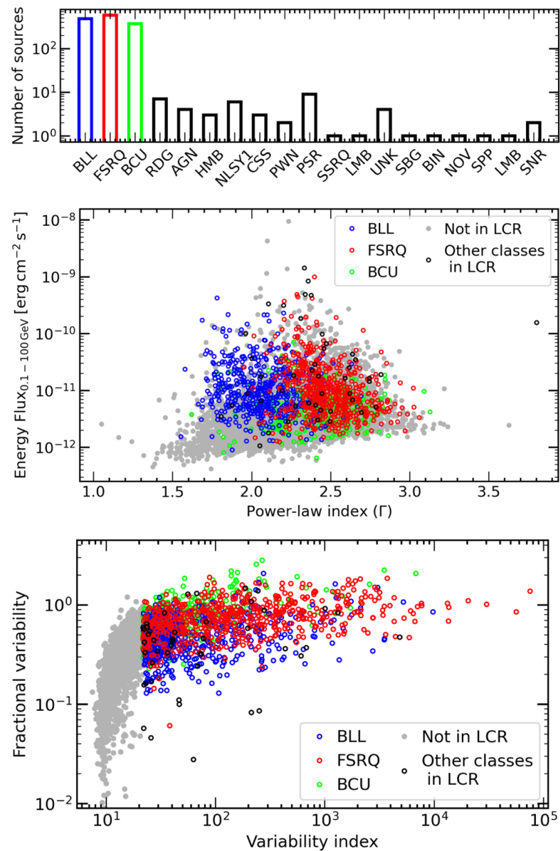
Figure 1. from S. Abdollahi et al 2023 Astrophys. J. Suppl. 265 doi:10.3847/1538-4365/acbb6a https://dx.doi.org/10.3847/1538-4365/acbb6a © 2023. The Author(s). Published by the American Astronomical Society.
