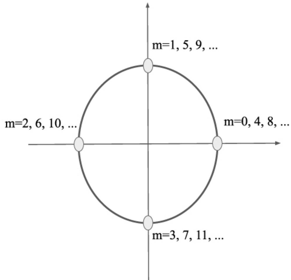
Figure 4. from Chi Tian et al 2022 Astrophys. J. Suppl. 263 doi:10.3847/1538-4365/ac958b https://dx.doi.org/10.3847/1538-4365/ac958b © 2022. The Author(s). Published by the American Astronomical Society.
