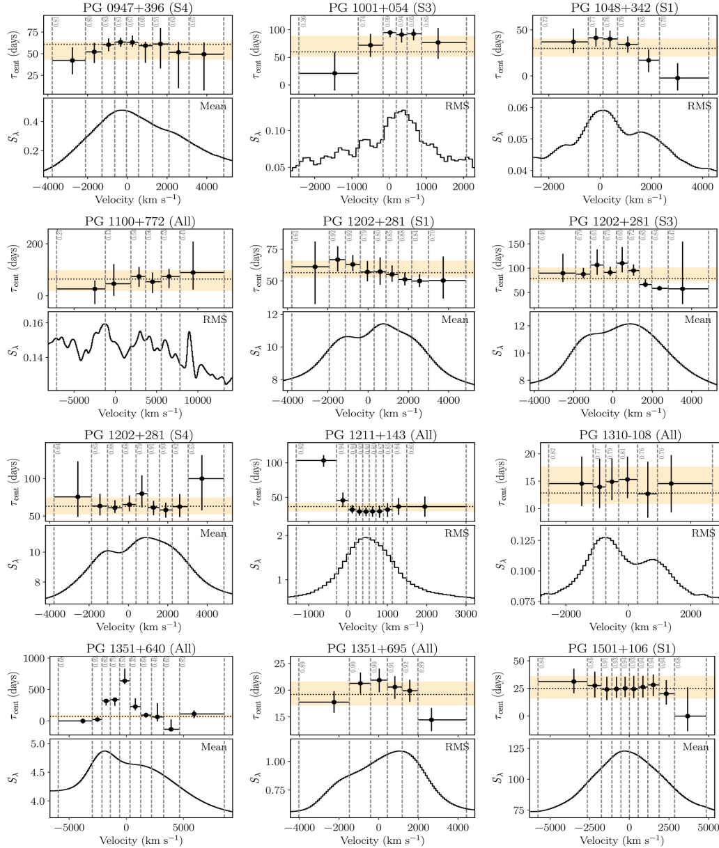
Figure 18. from Dong-Wei Bao et al 2022 Astrophys. J. Suppl. 262 doi:10.3847/1538-4365/ac7beb https://dx.doi.org/10.3847/1538-4365/ac7beb © 2022. The Author(s). Published by the American Astronomical Society.
