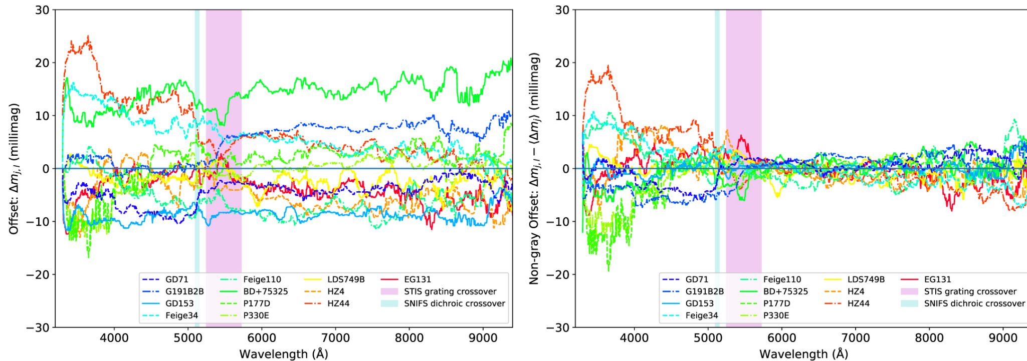
Figure 9. from David Rubin et al 2022 Astrophys. J. Suppl. 263 doi:10.3847/1538-4365/ac7b7f https://dx.doi.org/10.3847/1538-4365/ac7b7f © 2022. The Author(s). Published by the American Astronomical Society.
