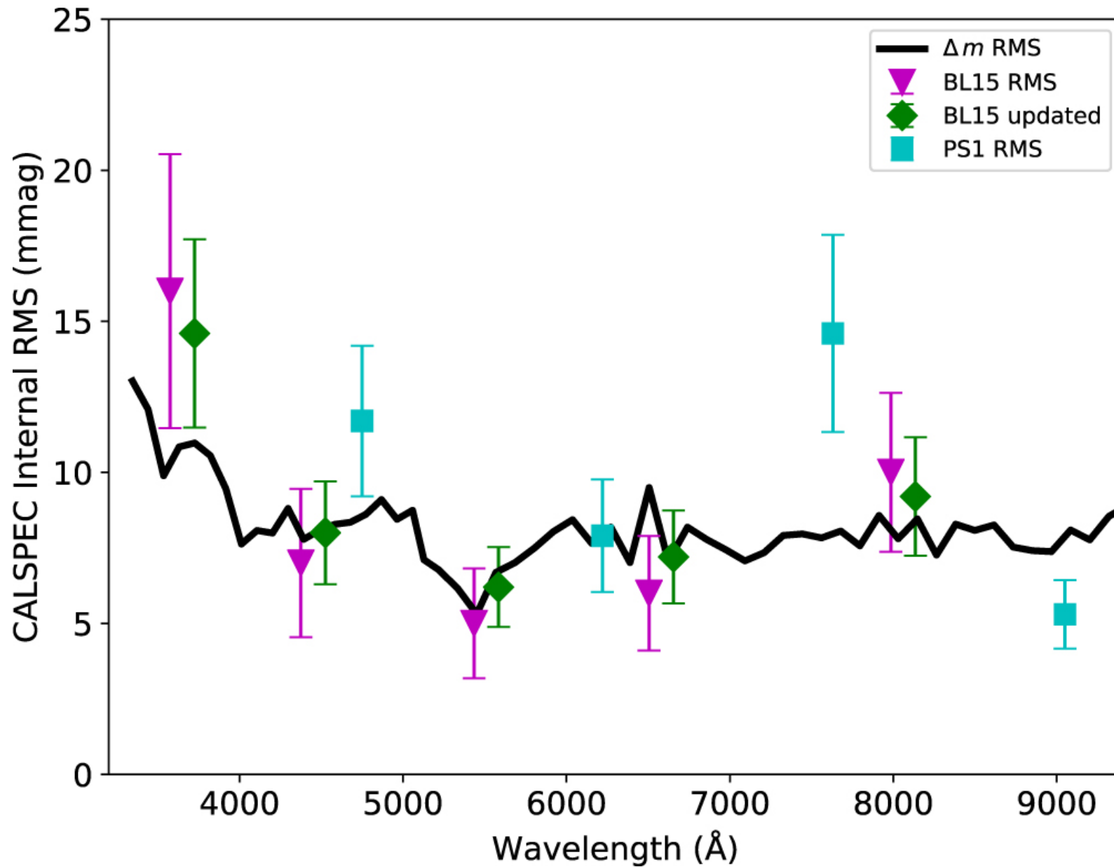
Figure 8. from David Rubin et al 2022 Astrophys. J. Suppl. 263 doi:10.3847/1538-4365/ac7b7f https://dx.doi.org/10.3847/1538-4365/ac7b7f © 2022. The Author(s). Published by the American Astronomical Society.
