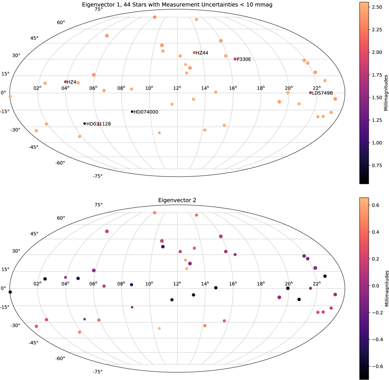
Figure 6. from David Rubin et al 2022 Astrophys. J. Suppl. 263 doi:10.3847/1538-4365/ac7b7f https://dx.doi.org/10.3847/1538-4365/ac7b7f © 2022. The Author(s). Published by the American Astronomical Society.
