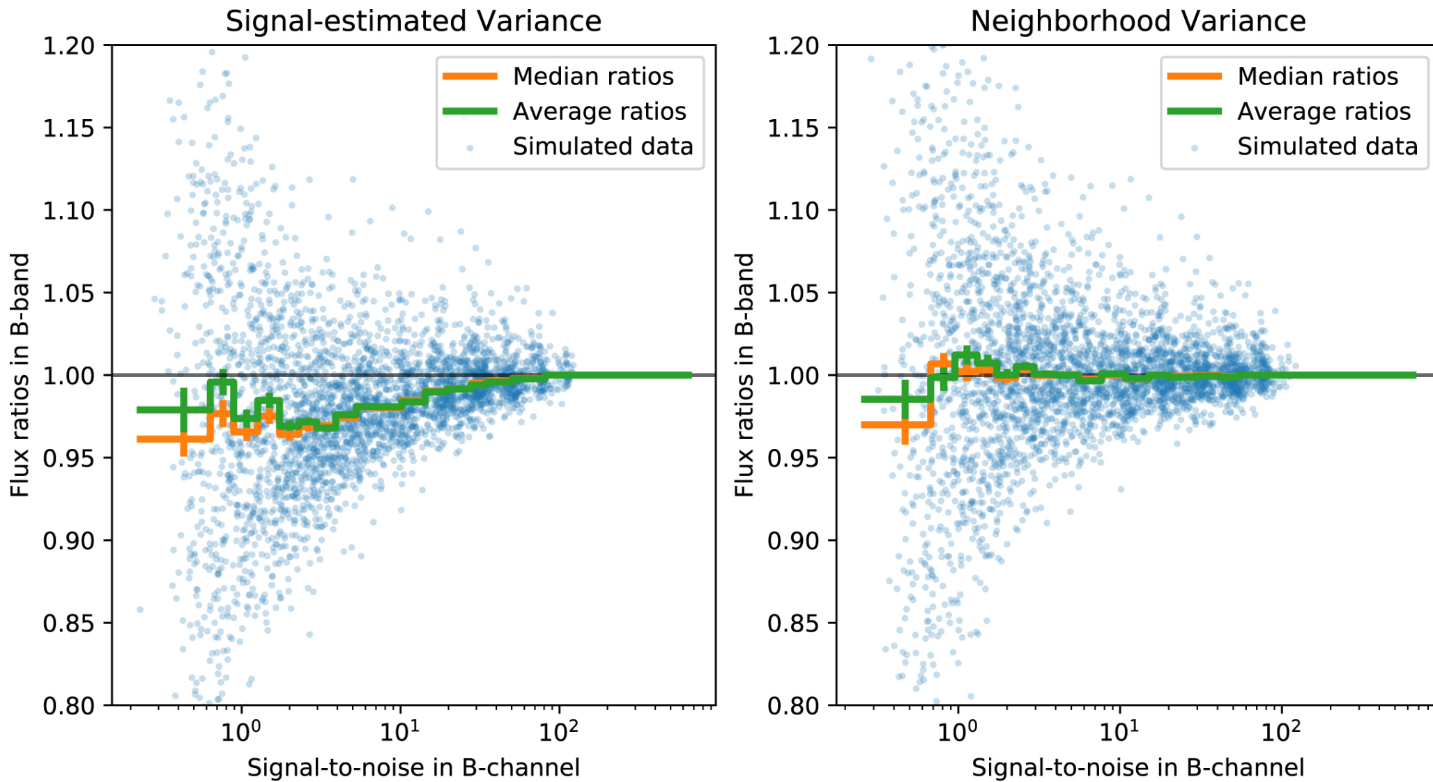
Figure 5. from David Rubin et al 2022 Astrophys. J. Suppl. 263 doi:10.3847/1538-4365/ac7b7f https://dx.doi.org/10.3847/1538-4365/ac7b7f © 2022. The Author(s). Published by the American Astronomical Society.
