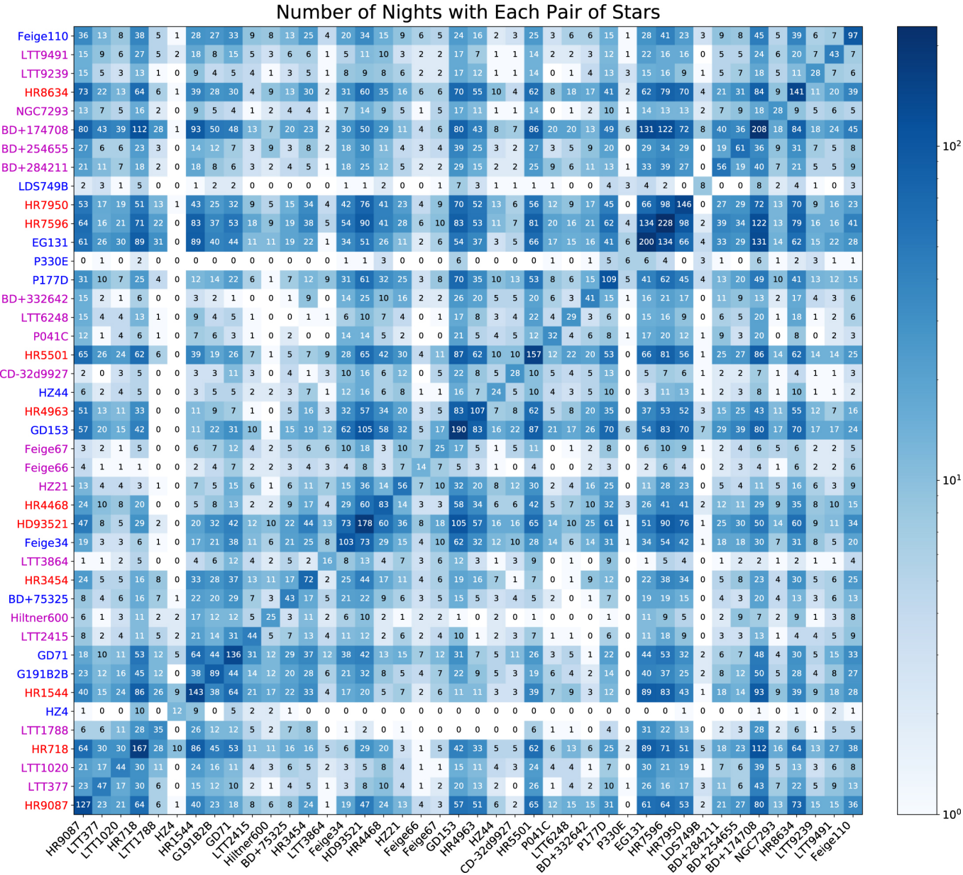
Figure 4. from David Rubin et al 2022 Astrophys. J. Suppl. 263 doi:10.3847/1538-4365/ac7b7f https://dx.doi.org/10.3847/1538-4365/ac7b7f © 2022. The Author(s). Published by the American Astronomical Society.
