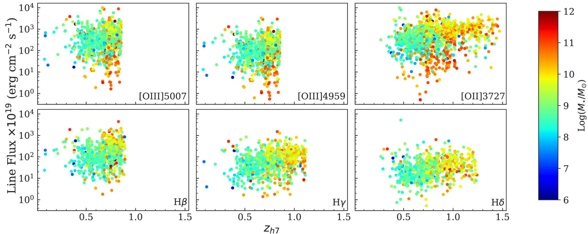
Figure 6. from John Pharo et al 2022 Astrophys. J. Suppl. 261 doi:10.3847/1538-4365/ac6cdf https://dx.doi.org/10.3847/1538-4365/ac6cdf © 2022. The Author(s). Published by the American Astronomical Society.
