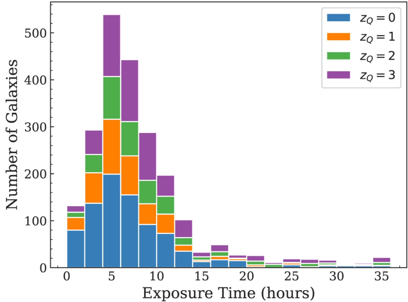
Figure 5. from John Pharo et al 2022 Astrophys. J. Suppl. 261 doi:10.3847/1538-4365/ac6cdf https://dx.doi.org/10.3847/1538-4365/ac6cdf © 2022. The Author(s). Published by the American Astronomical Society.
