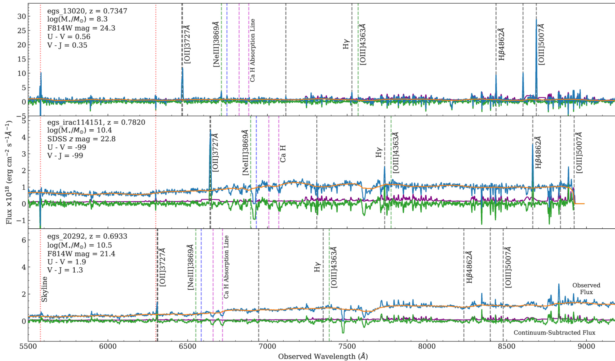
Figure 2. from John Pharo et al 2022 Astrophys. J. Suppl. 261 doi:10.3847/1538-4365/ac6cdf https://dx.doi.org/10.3847/1538-4365/ac6cdf © 2022. The Author(s). Published by the American Astronomical Society.
