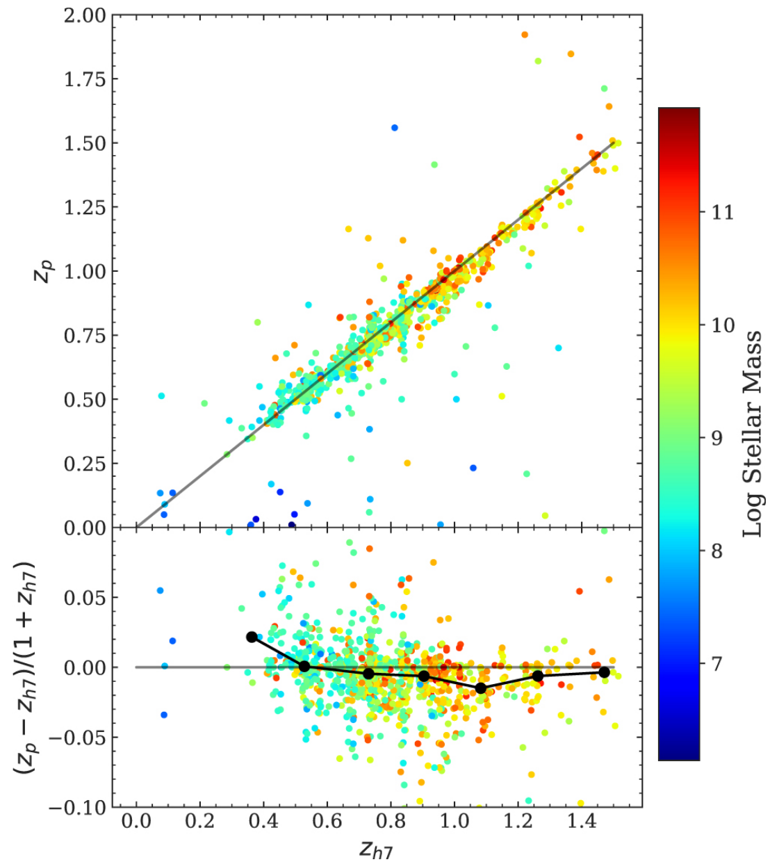
Figure 10. from John Pharo et al 2022 Astrophys. J. Suppl. 261 doi:10.3847/1538-4365/ac6cdf https://dx.doi.org/10.3847/1538-4365/ac6cdf © 2022. The Author(s). Published by the American Astronomical Society.
