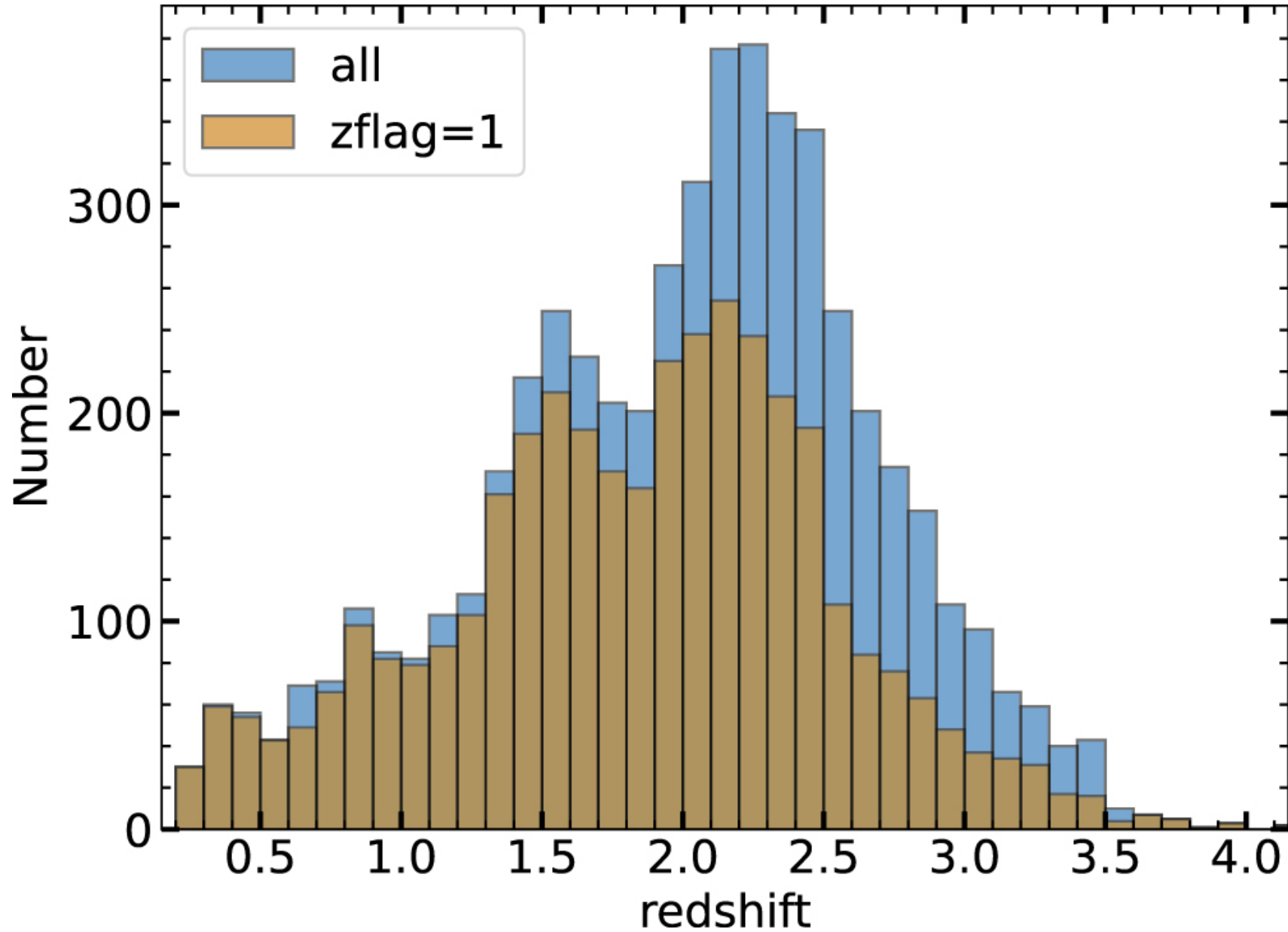
Figure 9. from Chenxu Liu et al 2022 Astrophys. J. Suppl. 261 doi:10.3847/1538-4365/ac6ba6 https://dx.doi.org/10.3847/1538-4365/ac6ba6 © 2022. The Author(s). Published by the American Astronomical Society.
