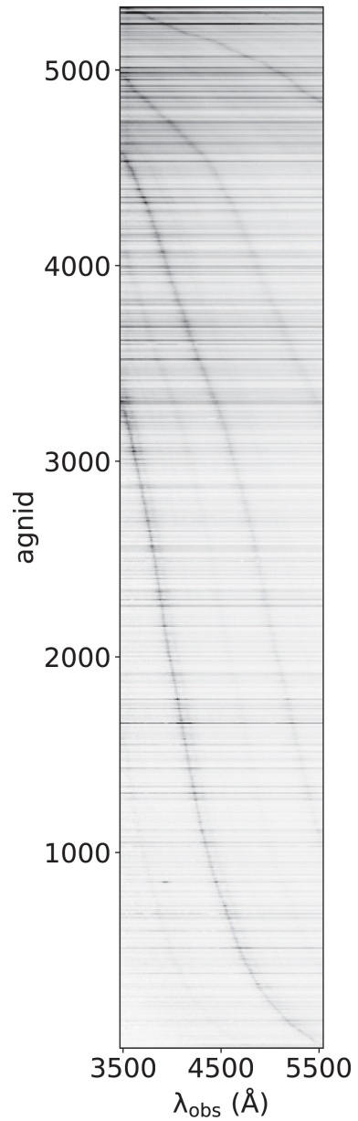
Figure 8. from Chenxu Liu et al 2022 Astrophys. J. Suppl. 261 doi:10.3847/1538-4365/ac6ba6 https://dx.doi.org/10.3847/1538-4365/ac6ba6 © 2022. The Author(s). Published by the American Astronomical Society.
