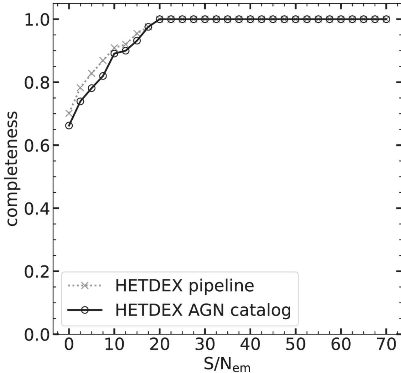
Figure 7. from Chenxu Liu et al 2022 Astrophys. J. Suppl. 261 doi:10.3847/1538-4365/ac6ba6 https://dx.doi.org/10.3847/1538-4365/ac6ba6 © 2022. The Author(s). Published by the American Astronomical Society.
