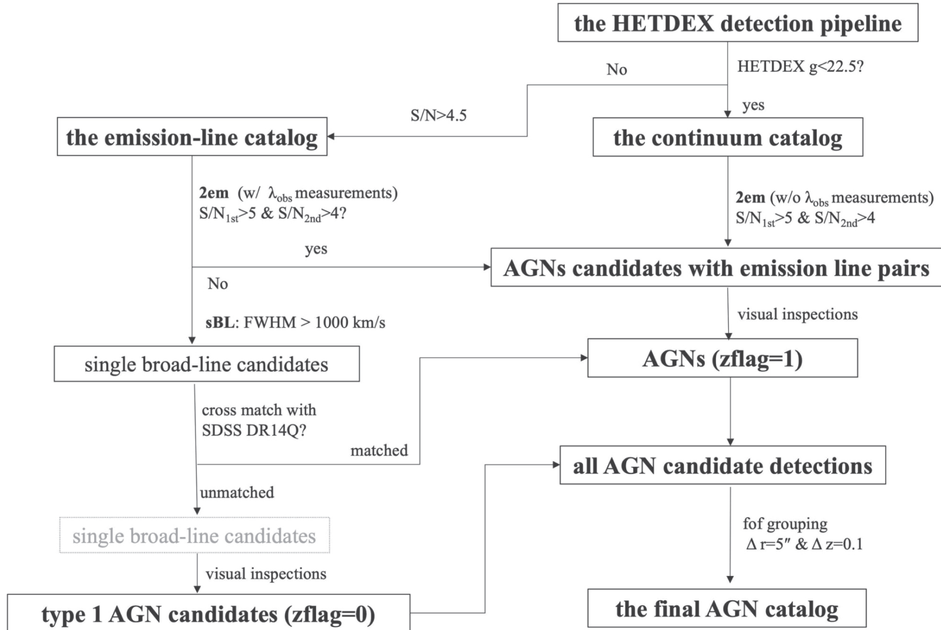
Figure 5. from Chenxu Liu et al 2022 Astrophys. J. Suppl. 261 doi:10.3847/1538-4365/ac6ba6 https://dx.doi.org/10.3847/1538-4365/ac6ba6 © 2022. The Author(s). Published by the American Astronomical Society.
