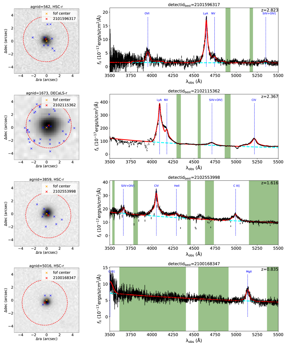
Figure 2. from Chenxu Liu et al 2022 Astrophys. J. Suppl. 261 doi:10.3847/1538-4365/ac6ba6 https://dx.doi.org/10.3847/1538-4365/ac6ba6 © 2022. The Author(s). Published by the American Astronomical Society.
