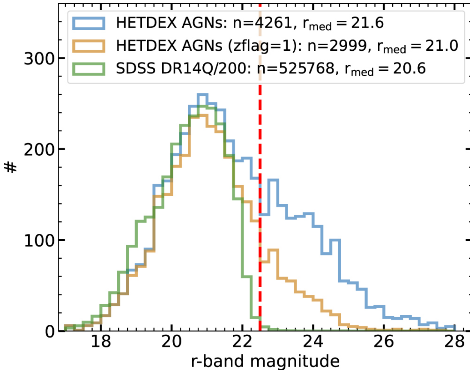
Figure 10. from Chenxu Liu et al 2022 Astrophys. J. Suppl. 261 doi:10.3847/1538-4365/ac6ba6 https://dx.doi.org/10.3847/1538-4365/ac6ba6 © 2022. The Author(s). Published by the American Astronomical Society.
