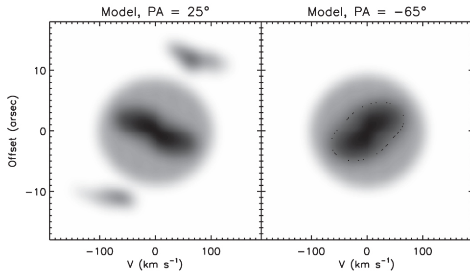
(c) Hb 4 Model ([N II] \lambda 6584 )
