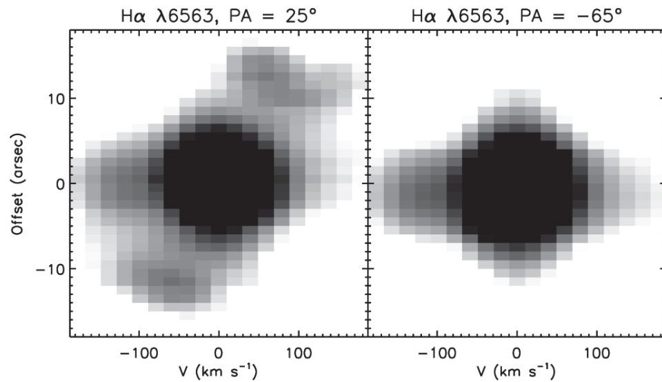
Figure 3. P–V arrays in the H 6563 and [N II] 6584 emissions from A. Danehkar 2022 Astrophys. J. Suppl. 260 doi:10.3847/1538-4365/ac5cca https://dx.doi.org/10.3847/1538-4365/ac5cca © 2022. The Author(s). Published by the American Astronomical Society.
