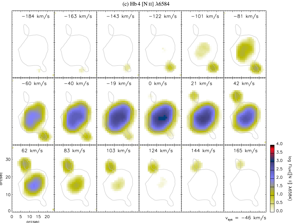
Figure 2. Velocity slices along the H 6563 and [N II] 6584 emission-line profiles from A. Danehkar 2022 Astrophys. J. Suppl. 260 doi:10.3847/1538-4365/ac5cca https://dx.doi.org/10.3847/1538-4365/ac5cca © 2022. The Author(s). Published by the American Astronomical Society.
