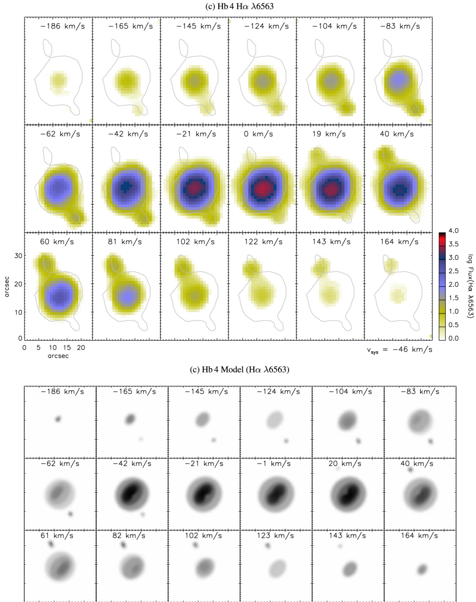
Figure 2. Velocity slices along the H 6563 and [N II] 6584 emission-line profiles from A. Danehkar 2022 Astrophys. J. Suppl. 260 doi:10.3847/1538-4365/ac5cca https://dx.doi.org/10.3847/1538-4365/ac5cca © 2022. The Author(s). Published by the American Astronomical Society.
