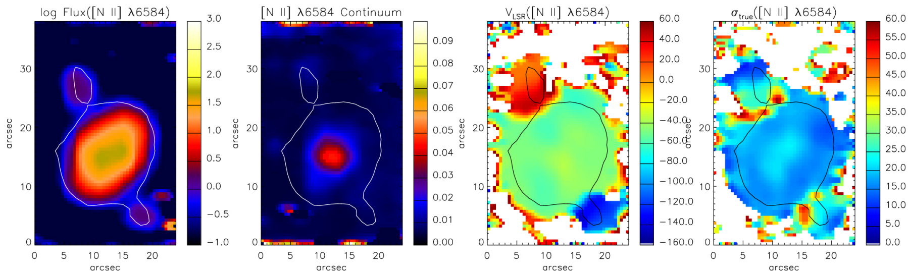
(c) Hb 4 [N II] \lambda 6584
