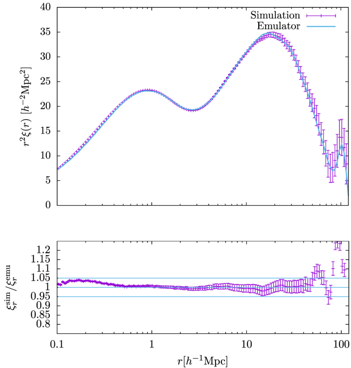
Figure 6. from Farpoint: A High-resolution Cosmology Simulation at the Gigaparsec Scale null 2022 APJS 259 15 doi:10.3847/1538-4365/ac43b9 https://dx.doi.org/10.3847/1538-4365/ac43b9 © 2022. The Author(s). Published by the American Astronomical Society.
