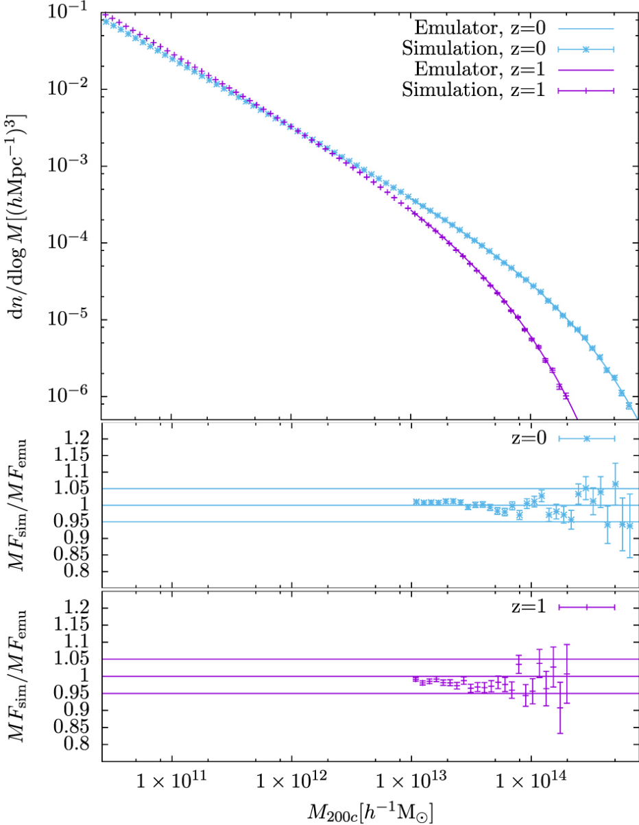
Figure 4. from Farpoint: A High-resolution Cosmology Simulation at the Gigaparsec Scale null 2022 APJS 259 15 doi:10.3847/1538-4365/ac43b9 https://dx.doi.org/10.3847/1538-4365/ac43b9 © 2022. The Author(s). Published by the American Astronomical Society.
