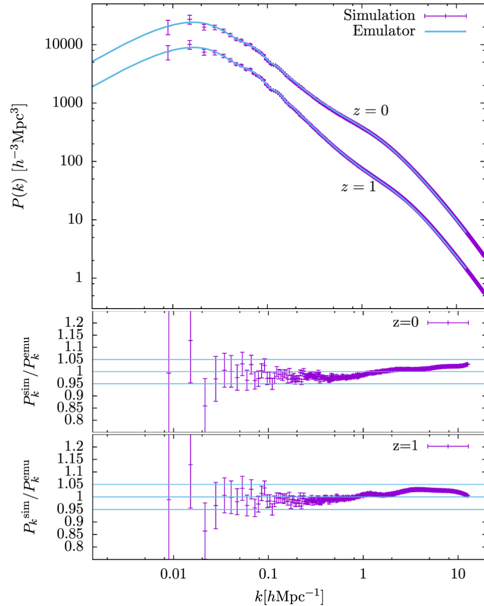
Figure 2. from Farpoint: A High-resolution Cosmology Simulation at the Gigaparsec Scale null 2022 APJS 259 15 doi:10.3847/1538-4365/ac43b9 https://dx.doi.org/10.3847/1538-4365/ac43b9 © 2022. The Author(s). Published by the American Astronomical Society.
