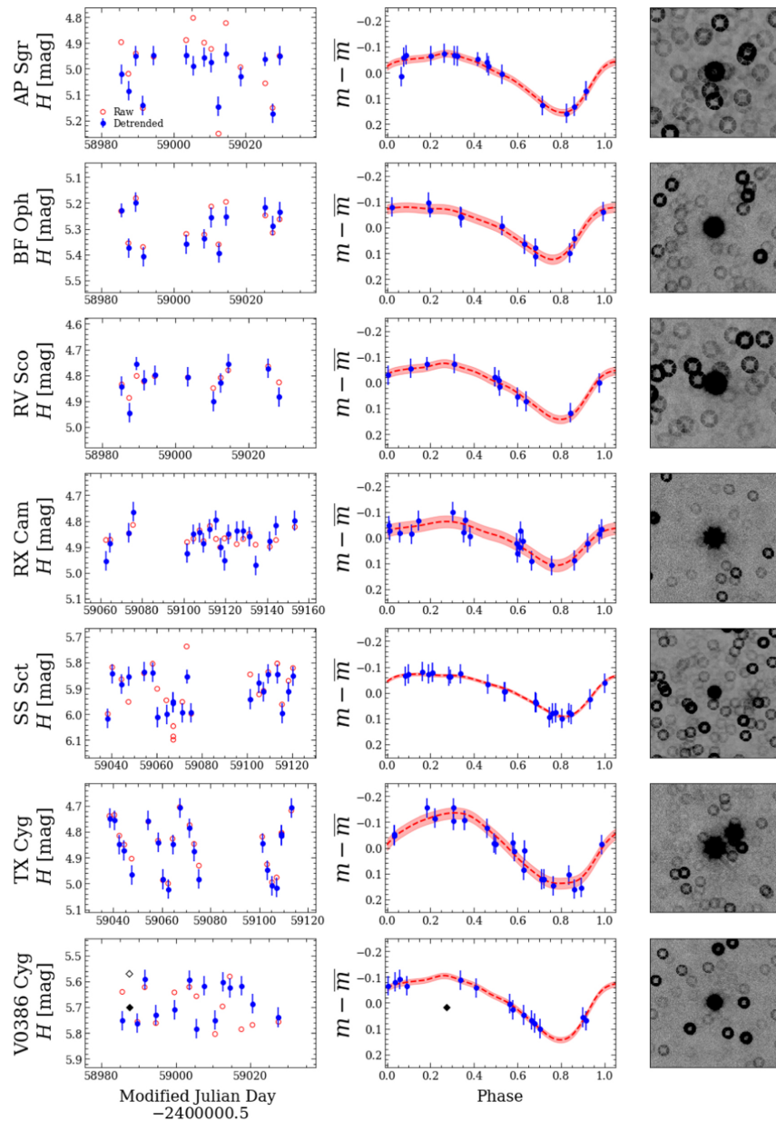
Figure 4. from H-band Light Curves of Milky Way Cepheids via Difference Imaging null 2022 APJS 258 24 doi:10.3847/1538-4365/ac41d3 https://dx.doi.org/10.3847/1538-4365/ac41d3 © 2022. The Author(s). Published by the American Astronomical Society.
