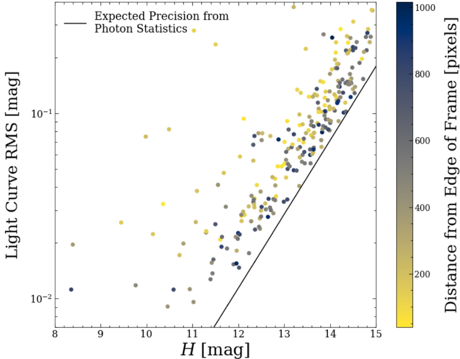
Figure 3. from H-band Light Curves of Milky Way Cepheids via Difference Imaging null 2022 APJS 258 24 doi:10.3847/1538-4365/ac41d3 https://dx.doi.org/10.3847/1538-4365/ac41d3 © 2022. The Author(s). Published by the American Astronomical Society.
