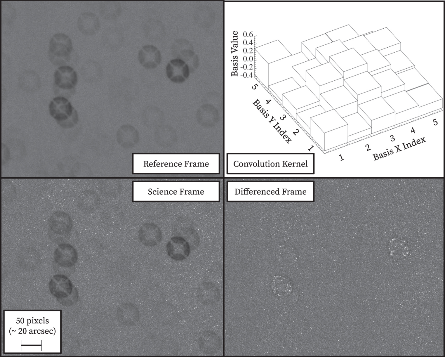
Figure 2. from H-band Light Curves of Milky Way Cepheids via Difference Imaging null 2022 APJS 258 24 doi:10.3847/1538-4365/ac41d3 https://dx.doi.org/10.3847/1538-4365/ac41d3 © 2022. The Author(s). Published by the American Astronomical Society.
