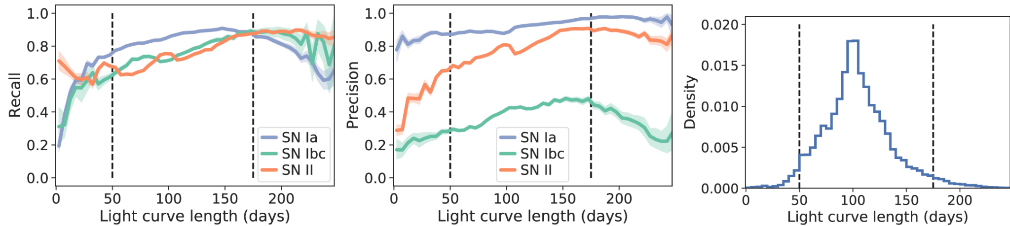
Figure 7. from Catarina S. Alves et al 2022 Astrophys. J. Suppl. 258 doi:10.3847/1538-4365/ac3479 https://dx.doi.org/10.3847/1538-4365/ac3479 © 2022. The Author(s). Published by the American Astronomical Society.
