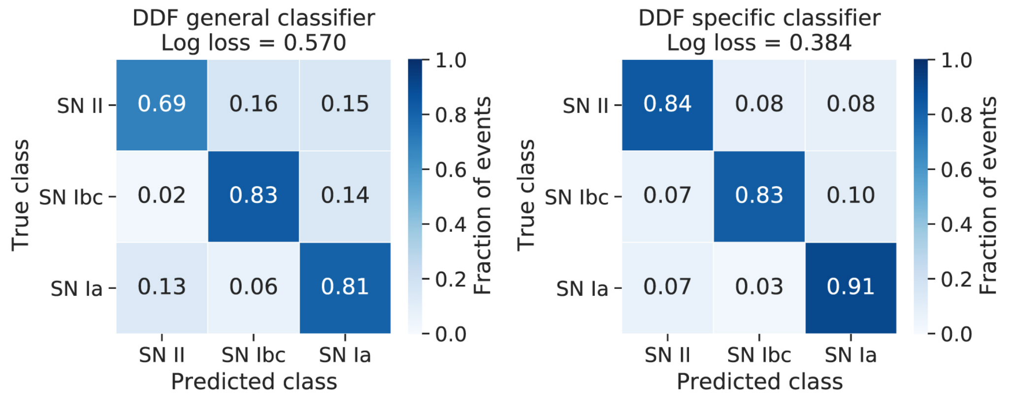
Figure 6. from Catarina S. Alves et al 2022 Astrophys. J. Suppl. 258 doi:10.3847/1538-4365/ac3479 https://dx.doi.org/10.3847/1538-4365/ac3479 © 2022. The Author(s). Published by the American Astronomical Society.
