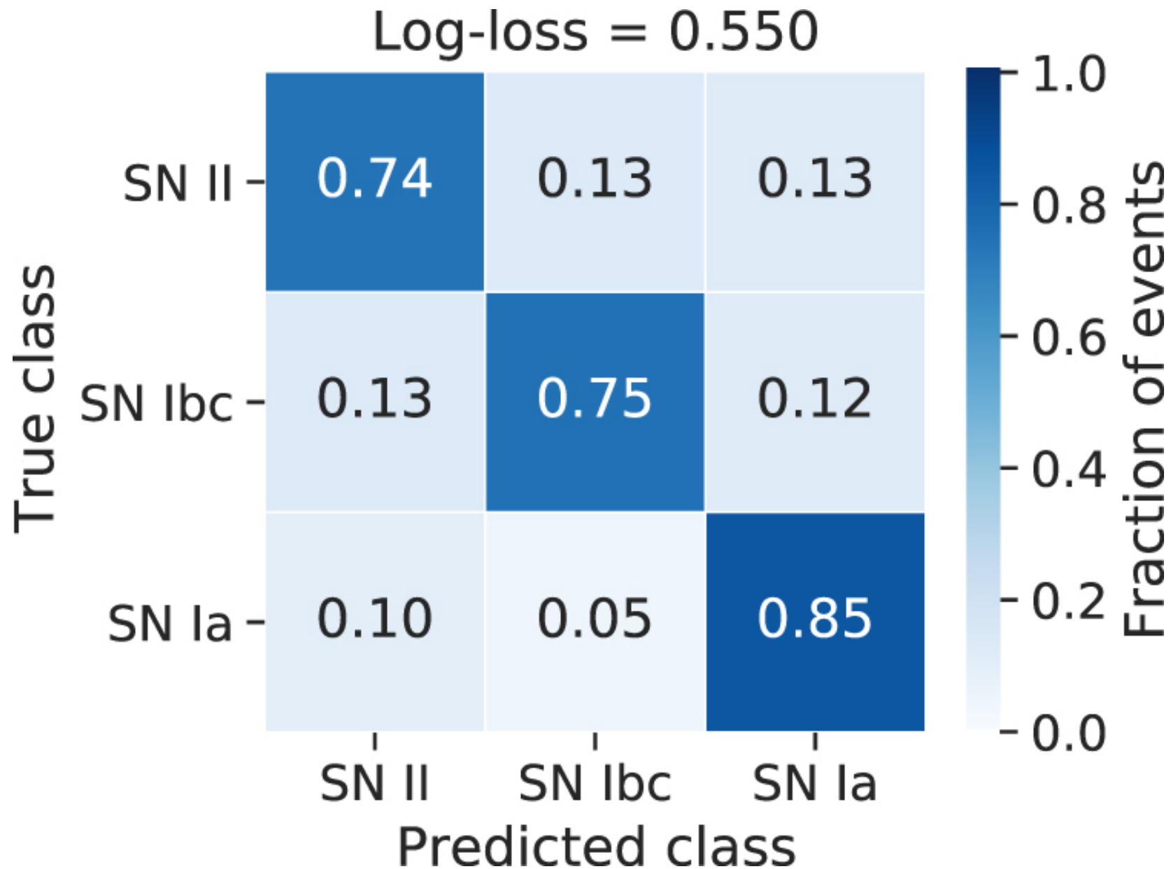
Figure 5. from Catarina S. Alves et al 2022 Astrophys. J. Suppl. 258 doi:10.3847/1538-4365/ac3479 https://dx.doi.org/10.3847/1538-4365/ac3479 © 2022. The Author(s). Published by the American Astronomical Society.
