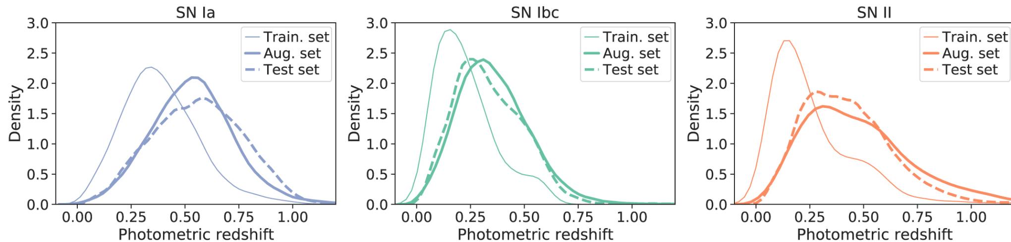
Figure 3. from Catarina S. Alves et al 2022 Astrophys. J. Suppl. 258 doi:10.3847/1538-4365/ac3479 https://dx.doi.org/10.3847/1538-4365/ac3479 © 2022. The Author(s). Published by the American Astronomical Society.
