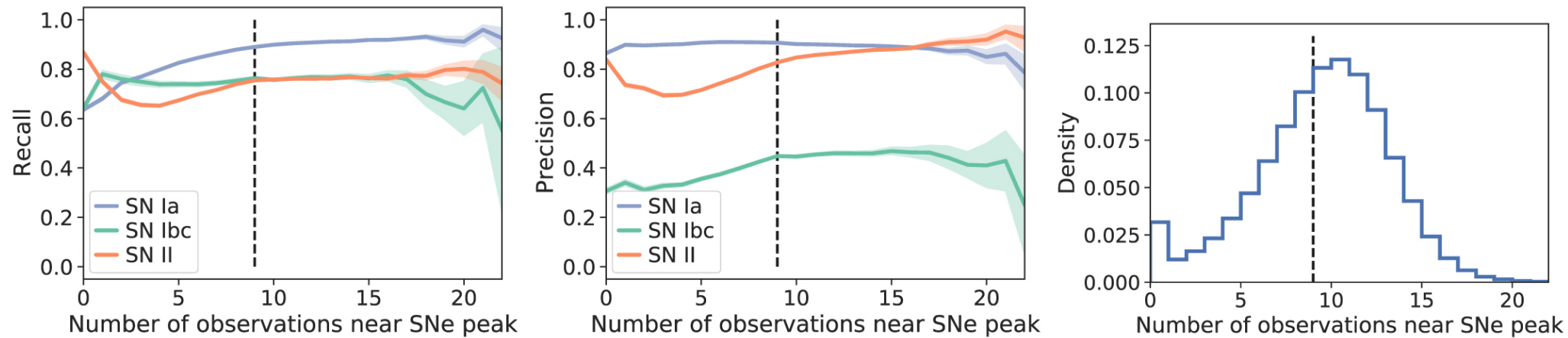
Figure 10. from Catarina S. Alves et al 2022 Astrophys. J. Suppl. 258 doi:10.3847/1538-4365/ac3479 https://dx.doi.org/10.3847/1538-4365/ac3479 © 2022. The Author(s). Published by the American Astronomical Society.
