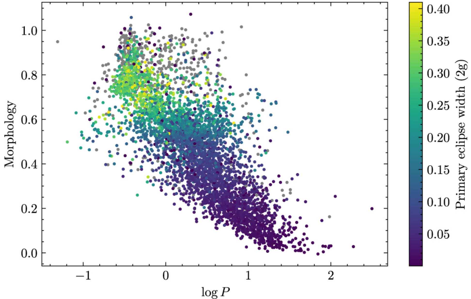
Figure 5. from TESS Eclipsing Binary Stars. I. Short-cadence Observations of 4584 Eclipsing Binaries in Sectors 1–26 null 2022 APJS 258 16 doi:10.3847/1538-4365/ac324a https://dx.doi.org/10.3847/1538-4365/ac324a © 2022. The Author(s). Published by the American Astronomical Society.
