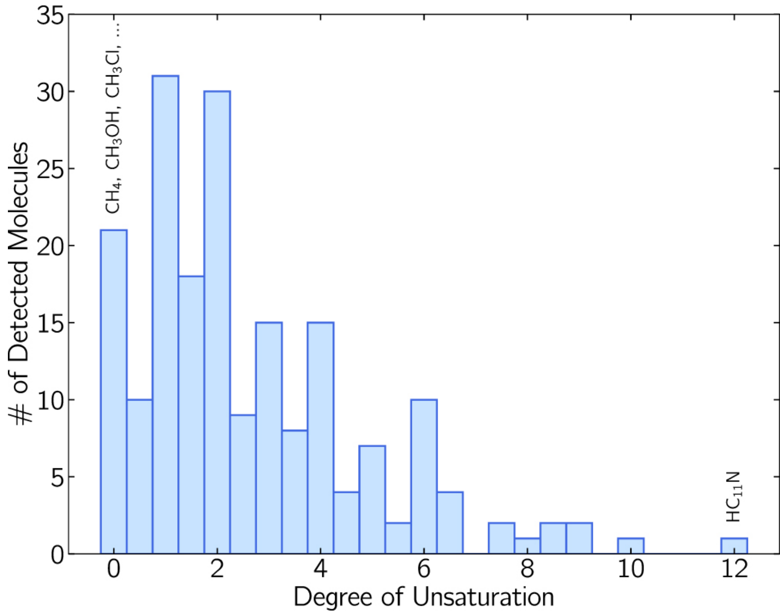
Figure 9. from 2021 Census of Interstellar, Circumstellar, Extragalactic, Protoplanetary Disk, and Exoplanetary Molecules null 2022 APJS 259 30 doi:10.3847/1538-4365/ac2a48 https://dx.doi.org/10.3847/1538-4365/ac2a48 © 2022. The Author(s). Published by the American Astronomical Society.
