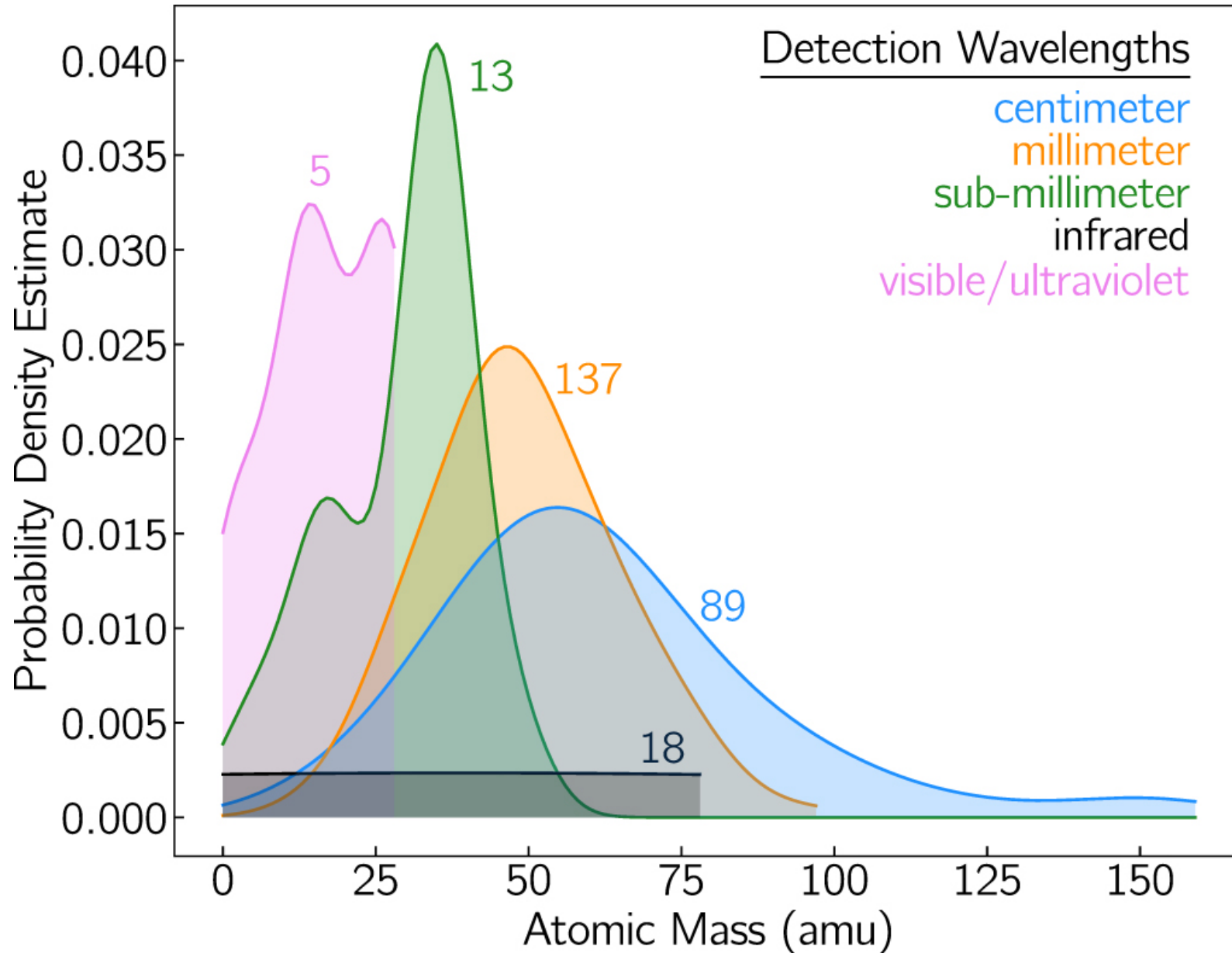
Figure 7. from 2021 Census of Interstellar, Circumstellar, Extragalactic, Protoplanetary Disk, and Exoplanetary Molecules null 2022 APJS 259 30 doi:10.3847/1538-4365/ac2a48 https://dx.doi.org/10.3847/1538-4365/ac2a48 © 2022. The Author(s). Published by the American Astronomical Society.
