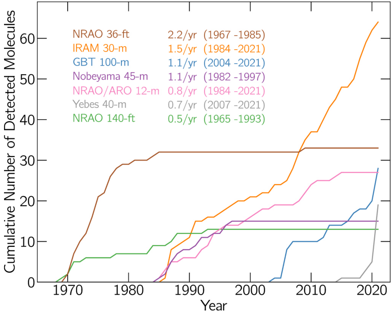
Figure 5. from 2021 Census of Interstellar, Circumstellar, Extragalactic, Protoplanetary Disk, and Exoplanetary Molecules null 2022 APJS 259 30 doi:10.3847/1538-4365/ac2a48 https://dx.doi.org/10.3847/1538-4365/ac2a48 © 2022. The Author(s). Published by the American Astronomical Society.
