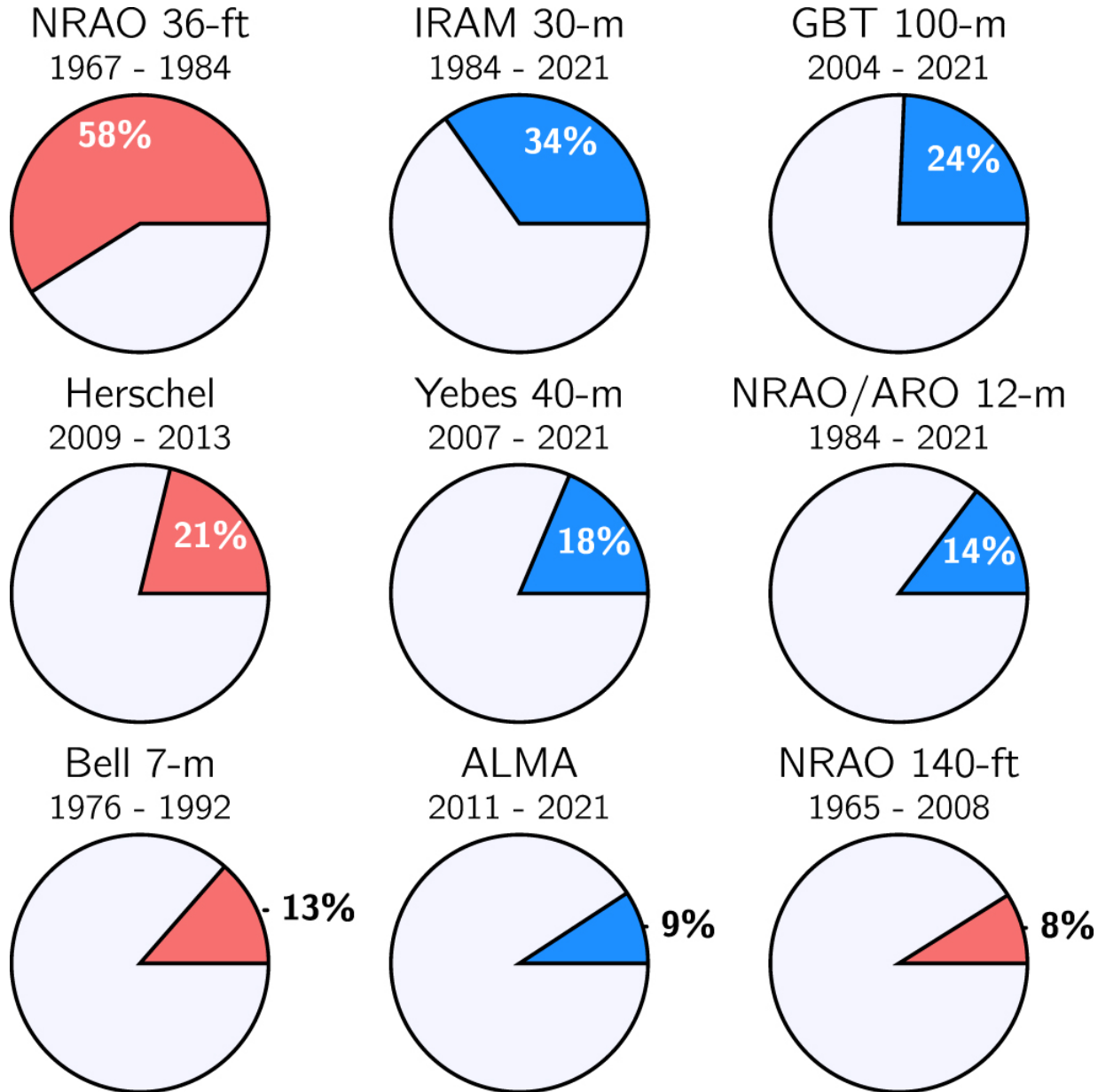
Figure 4. from 2021 Census of Interstellar, Circumstellar, Extragalactic, Protoplanetary Disk, and Exoplanetary Molecules null 2022 APJS 259 30 doi:10.3847/1538-4365/ac2a48 https://dx.doi.org/10.3847/1538-4365/ac2a48
