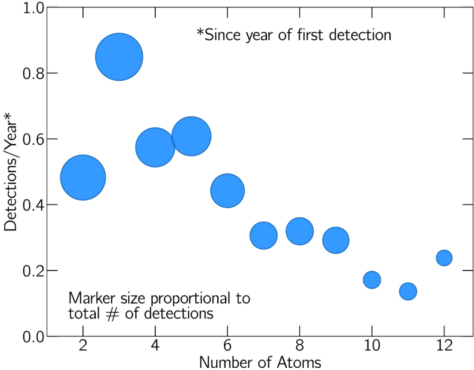
Figure 3. from 2021 Census of Interstellar, Circumstellar, Extragalactic, Protoplanetary Disk, and Exoplanetary Molecules null 2022 APJS 259 30 doi:10.3847/1538-4365/ac2a48 https://dx.doi.org/10.3847/1538-4365/ac2a48 © 2022. The Author(s). Published by the American Astronomical Society.
