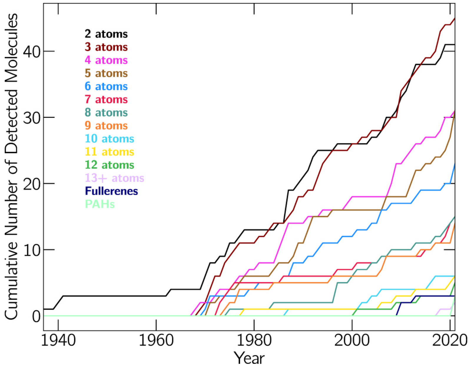
Figure 2. from 2021 Census of Interstellar, Circumstellar, Extragalactic, Protoplanetary Disk, and Exoplanetary Molecules null 2022 APJS 259 30 doi:10.3847/1538-4365/ac2a48 https://dx.doi.org/10.3847/1538-4365/ac2a48 © 2022. The Author(s). Published by the American Astronomical Society.
