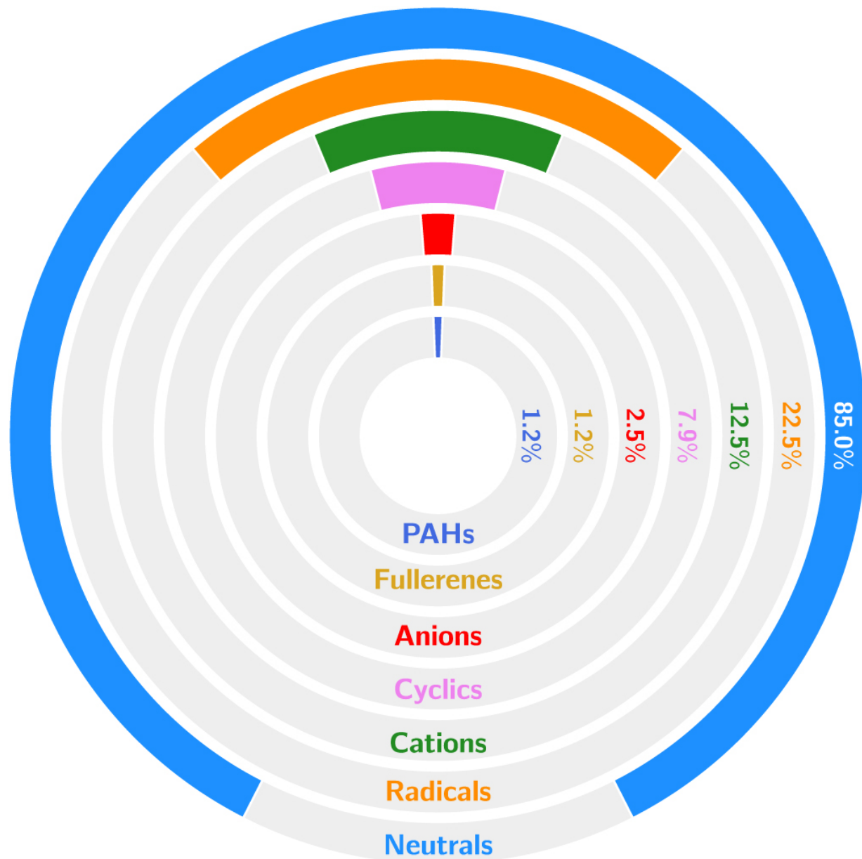
Figure 10. from 2021 Census of Interstellar, Circumstellar, Extragalactic, Protoplanetary Disk, and Exoplanetary Molecules null 2022 APJS 259 30 doi:10.3847/1538-4365/ac2a48 https://dx.doi.org/10.3847/1538-4365/ac2a48 © 2022. The Author(s). Published by the American Astronomical Society.
