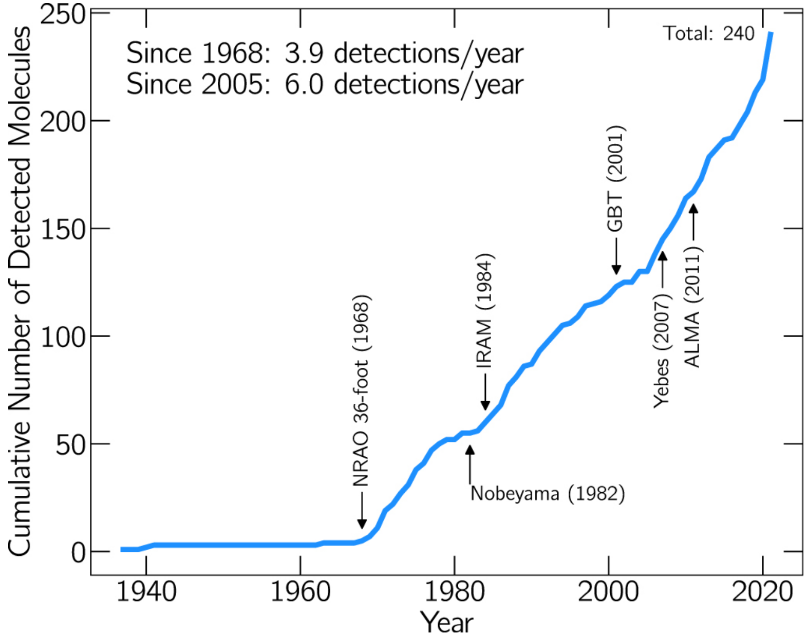
Figure 1. from 2021 Census of Interstellar, Circumstellar, Extragalactic, Protoplanetary Disk, and Exoplanetary Molecules null 2022 APJS 259 30 doi:10.3847/1538-4365/ac2a48 https://dx.doi.org/10.3847/1538-4365/ac2a48 © 2022. The Author(s). Published by the American Astronomical Society.
