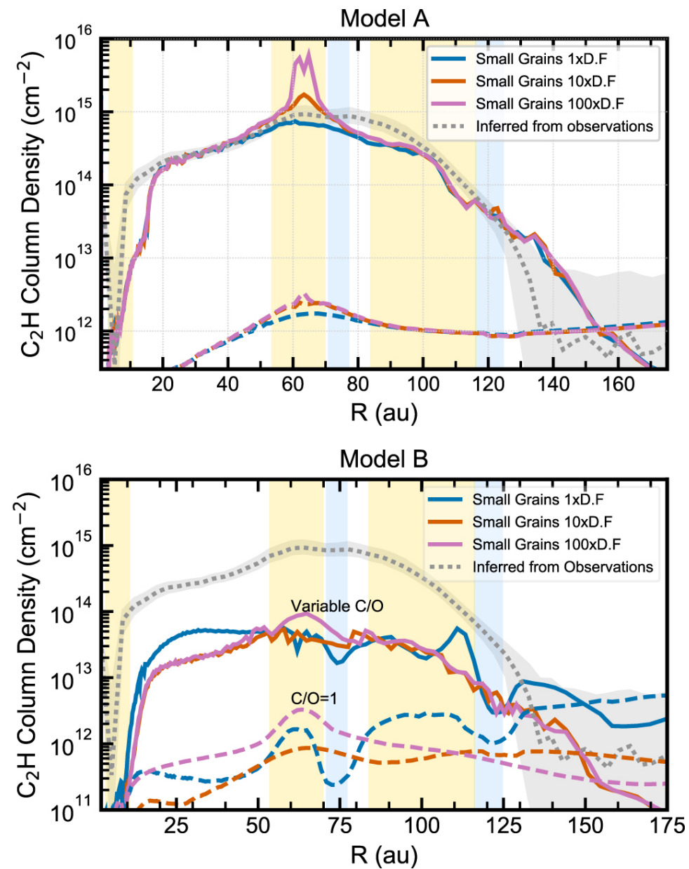
Figure 9. from Felipe Alarcón et al 2021 Astrophys. J. Suppl. 257 doi:10.3847/1538-4365/ac22ae https://dx.doi.org/10.3847/1538-4365/ac22ae © 2021. The American Astronomical Society. All rights reserved.
