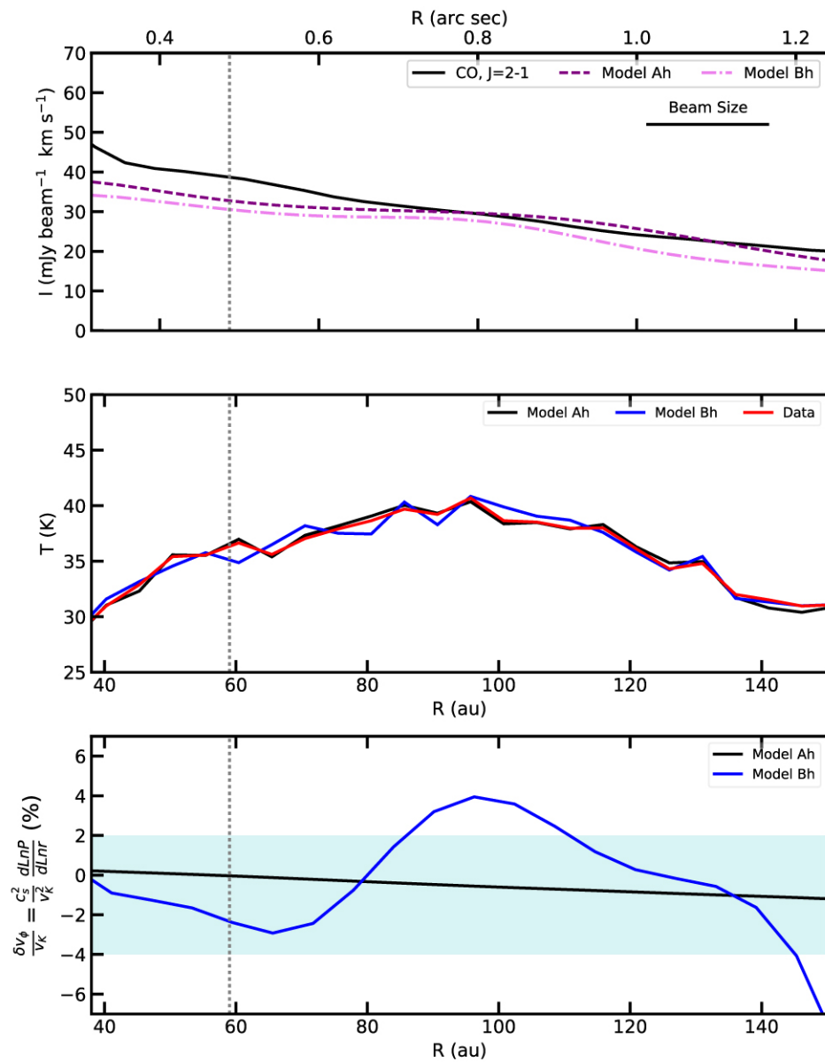
Figure 8. from Felipe Alarcón et al 2021 Astrophys. J. Suppl. 257 doi:10.3847/1538-4365/ac22ae https://dx.doi.org/10.3847/1538-4365/ac22ae © 2021. The American Astronomical Society. All rights reserved.
