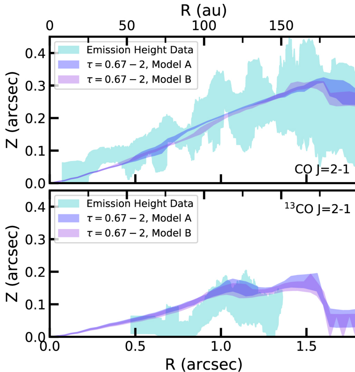
Figure 5. from Felipe Alarcón et al 2021 Astrophys. J. Suppl. 257 doi:10.3847/1538-4365/ac22ae https://dx.doi.org/10.3847/1538-4365/ac22ae © 2021. The American Astronomical Society. All rights reserved.
